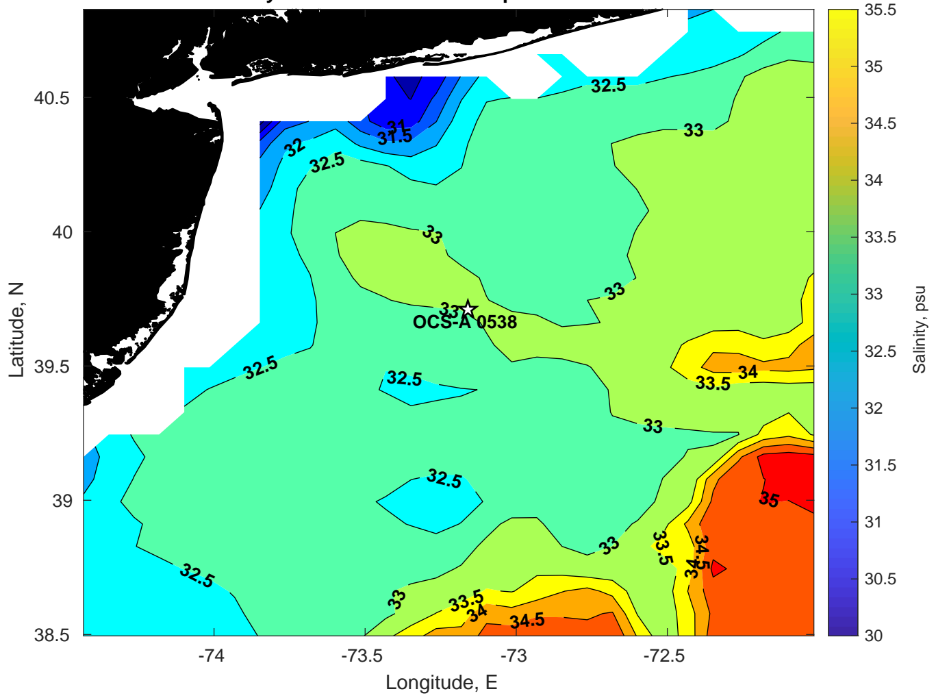
Surface Salinity for OCS-A 0538 at 18-Apr-2024 00:00:00
